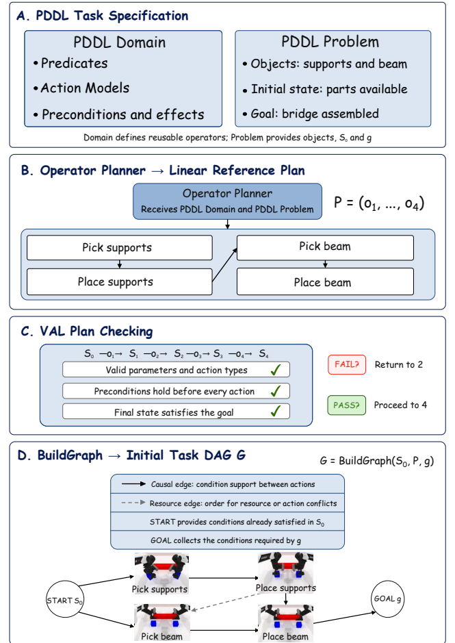
Fig. 2. LOGIV pre-execution planning and task-graph construction. The Operator Planner generates the reference plan P , where each o_i in panel (B) is a grounded high-level PDDL operator. After validation by VAL, P is compiled into the initial task graph G .
