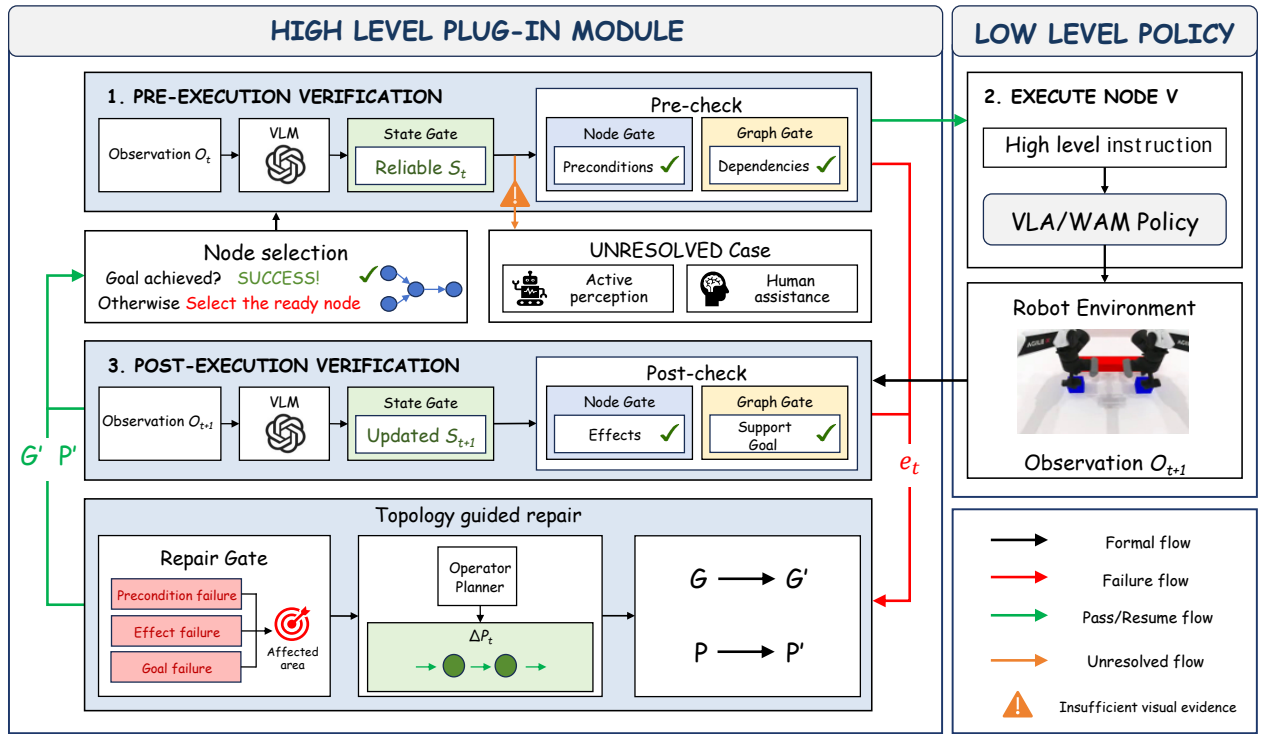
Fig. 3. LOGIV online verification and topology-guided causal local repair. The three gates establish reliable task facts, verify the selected subtask, and check graph dependencies. Upon a failure, the Repair Gate identifies affected nodes, validates a local repair plan, rebuilds the task graph, and resumes execution. Human assistance is reserved for future evaluation.
