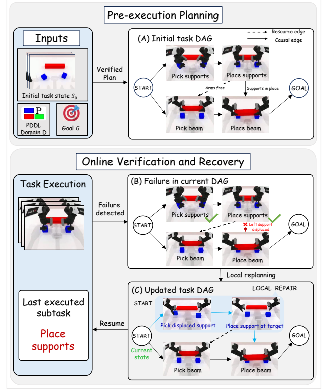
Fig. 1. LOGIV execution on the BiCoord build_bridge task. (A) A validated reference plan is compiled into the initial task DAG before execution. (B) A previously placed support is displaced, invalidating a condition required by the remaining plan. (C) LOGIV repairs only the affected support operations, retains the unaffected beam operations, and resumes execution on the updated task DAG.
