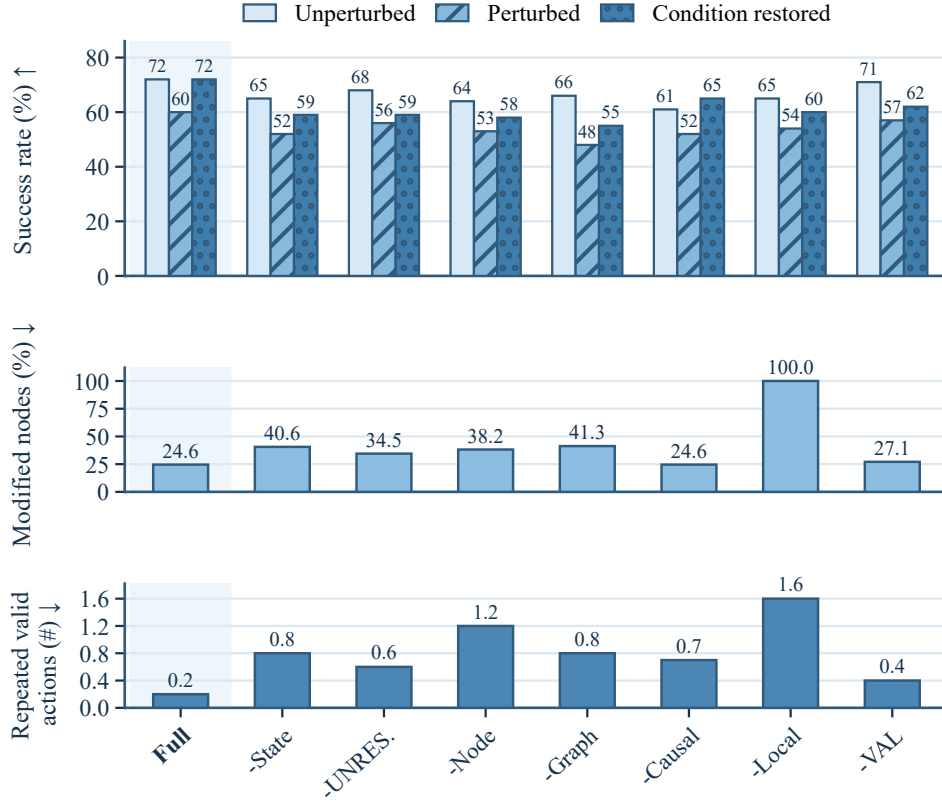
Fig. 5. Ablation results of LOGIV. The top panel shows task completion and condition restoration under perturbations. The middle and bottom panels show modified nodes and repeated valid actions during repair, respectively. Full: complete method; -State: no State Gate; -UNRES: no uncertainty handling; -Node: no Node Gate; -Graph: no Graph Gate; -Causal: no causal dependency tracing; -Local: replanning all remaining actions instead of local repair; -VAL: no logical validation of the repaired plan.
